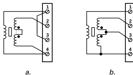
Figure 3. Four-Wire LVDT Connections
