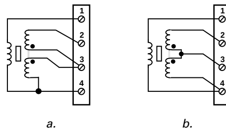
Figure 4. Five-Wire LVDT Connections
