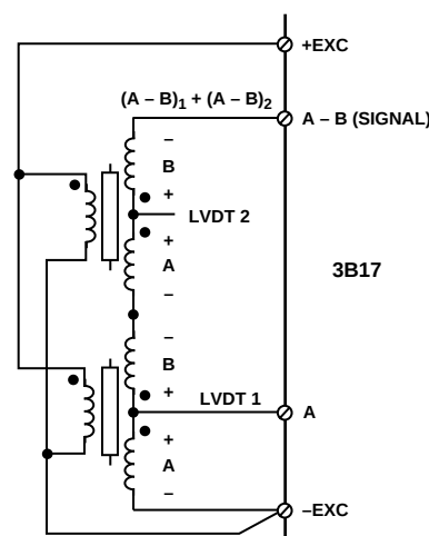
Figure 1. Additive LVDT Connections
